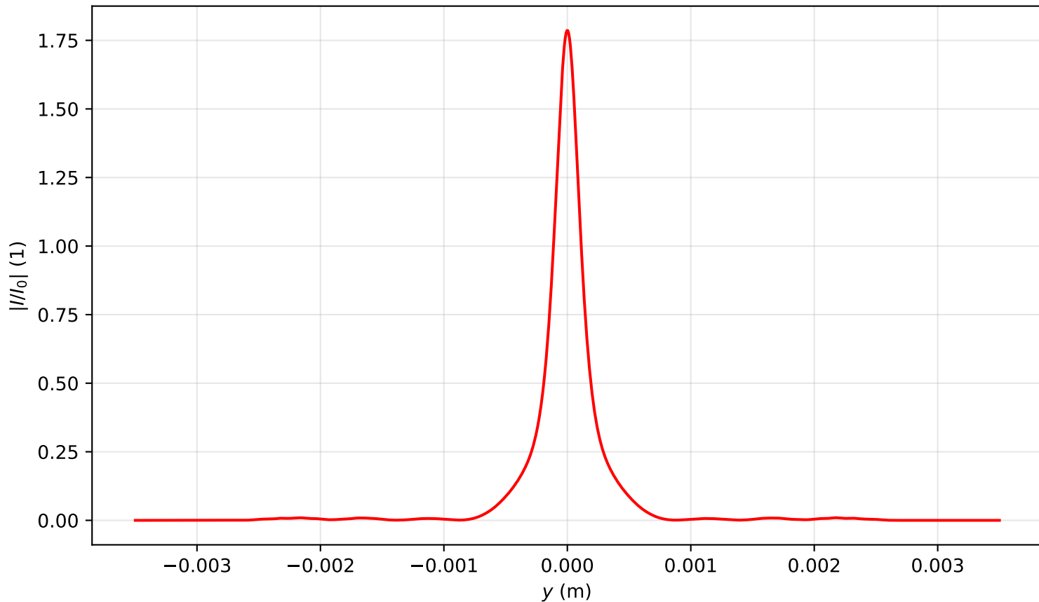
Intensity profile I(x=0, y, z=0.955)/I_0 , P_{in}=4.0P_{cr} , artificial time
